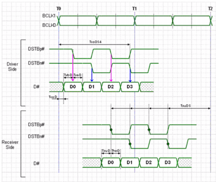
Data Bus Timing Diagram ©Intel Corporation
