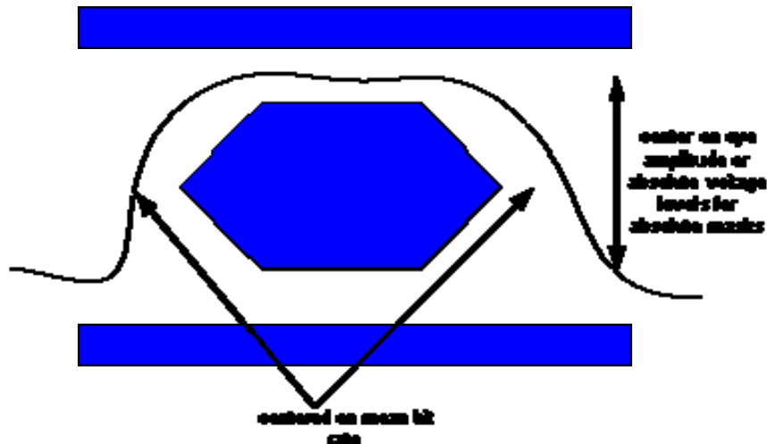
Figure 4. Eye Mask Alignment for Violation Locator
